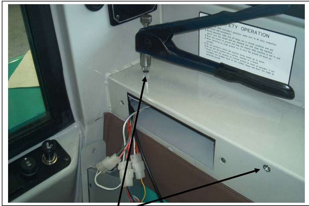
2 of four holes drilled with threaded insert for securing the evaporator
